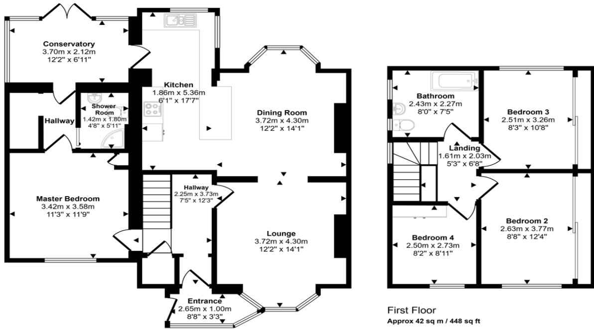
Ground Floor Approx 84 sq m / 904 sq ft
